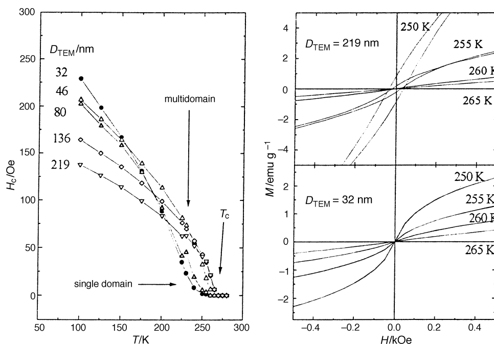
Fig. 13 Coercive fields of the sol-gel samples measured between 100 and 300 K, obtained from the hysteresis loops. Each sample is labelled after the average particle size obtained by transmission electron microscopy.
