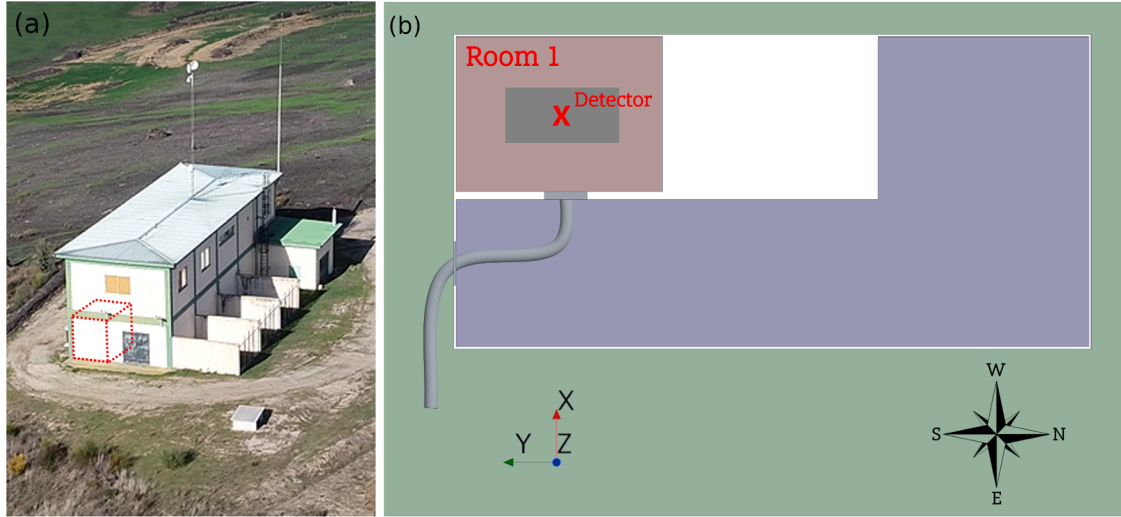
Fig. 1. (a) Aerial view of the LNR, showing the studied room marked in red. (b) Reconstructed geometry of the LNR building inside the simulation software. The detector position is marked with a red cross, and the system used in the mechanical ventilation simulation is shown with a gray tube. (For interpretation of the references to colour in this figure legend, the reader is referred to the web version of this article.)
